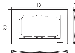
Frame for Double Socket
