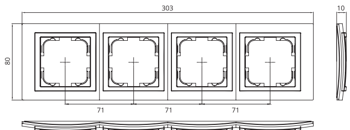
4 Gang Frame
