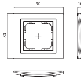
Single Frame
