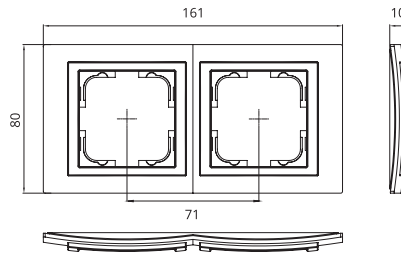
Double Frame
