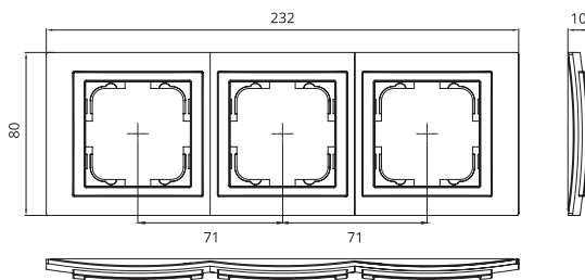
Triple Frame
